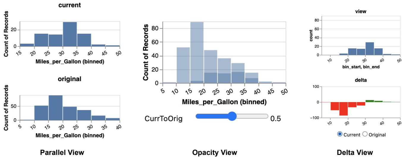
Figure 4: DITL uses three approaches for rendering data differences: parallel view, opacity view, and delta view.
