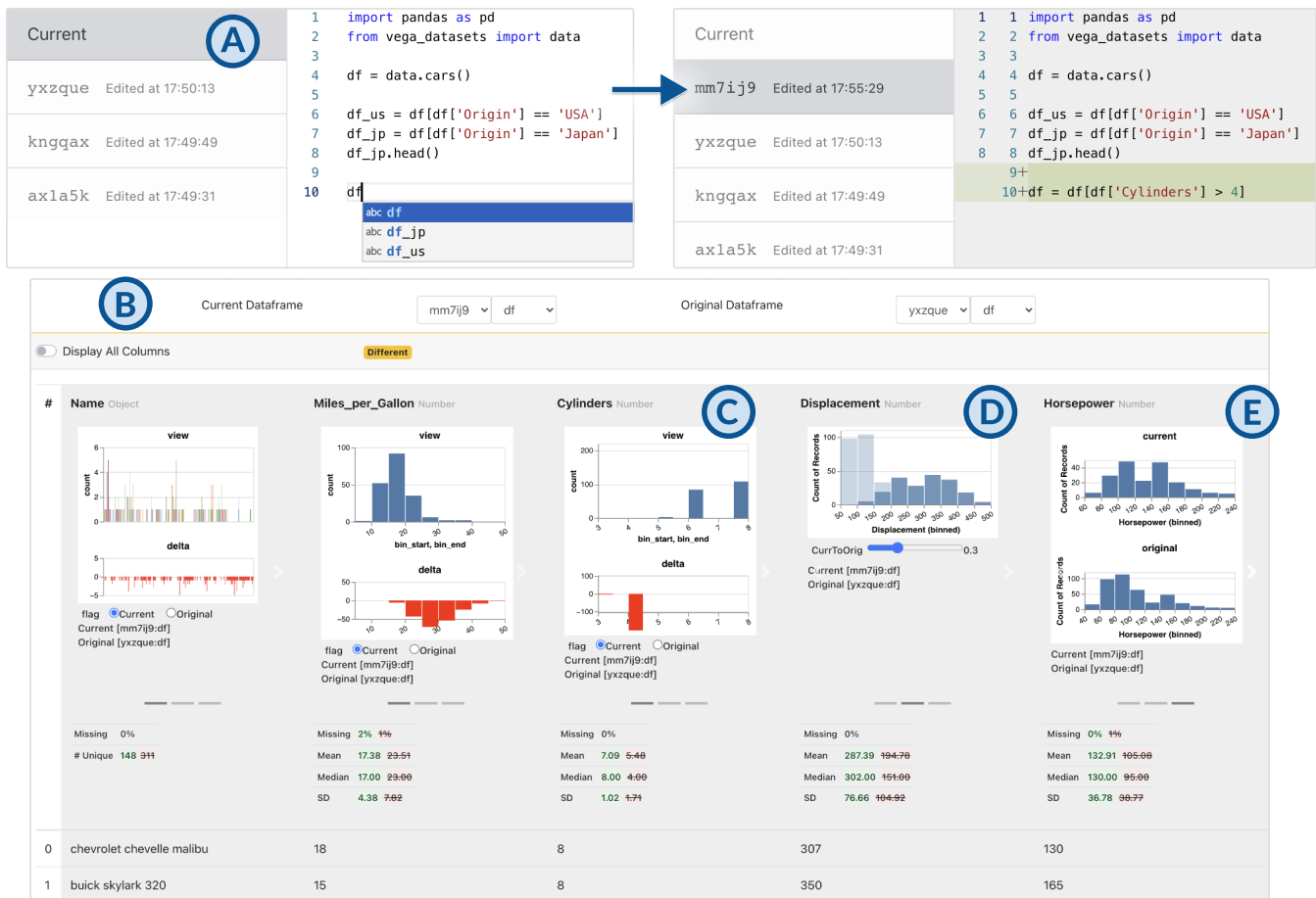
Figure 1: As users iterate on their data during analysis, they can use DITL to compare data snapshots. Every time users successfully execute code we save a snapshot (A). Users can compare the code using traditional code diffing tools. Users can also use DITL to compare data iterations with interactive visualizations, descriptive statistics, and data preview (B). User can choose three ways to visualize the differences in each column: delta view (C), opacity view (D), and parallel view (E).
