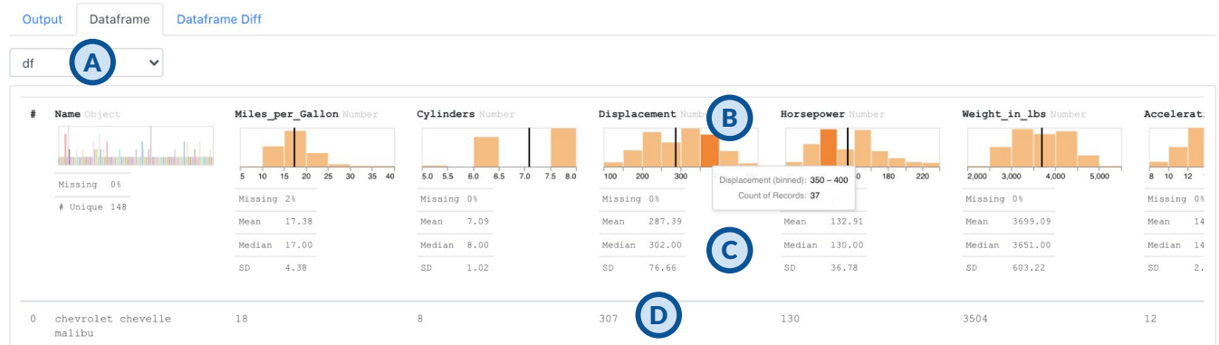
Figure 3: The data panel allows users to inspect a single data table. (A) Users can select saved data frames from the current code snapshot; (B) The data panel shows the distribution of each column; (C) The data panel shows the summary statistics for each column; (D) The data panel shows a sample of rows from the selected data frame.
