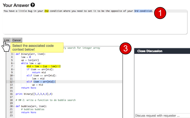
Fig. 2. The contextualized explanation feature and the chat tool. To make their answers more contextualized, instructors can (1) select a portion of the text in their natural language answer and the relevant code context; (2) click the ‘link’ button to create the references, which will highlight the relevant code (hypertext) when clicking the references in the text. Instructors can also chat with students via (3).
